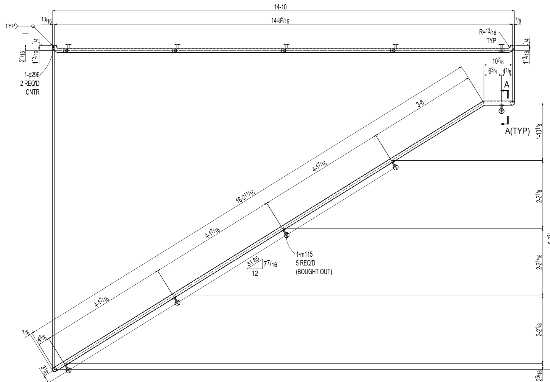
ONE WALLRAIL 4032WR1
